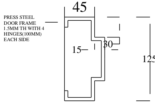
SEC AT B-B
