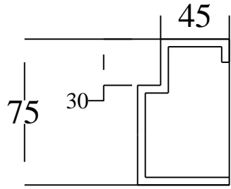
SEC OF FRAME (CHOWKAT) FOR W/O FLY PROOF SHUTTER
