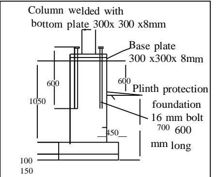
450 x 450 PCC COLUMN FOUNDATION
