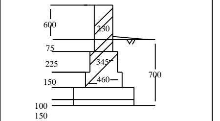
PLINTH/DRAFT WALL FOUNDATION
