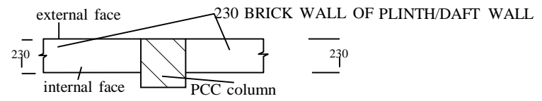
450 x 450 PCC COLUMN FOUNDATION WITH PLINTH WALL
